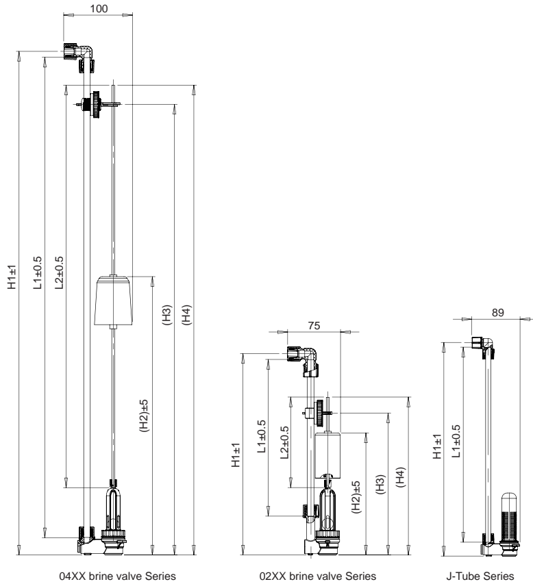
04XX brine valve Series
