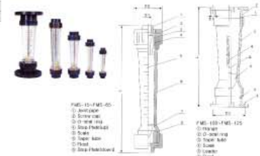
The drawing and installation size of FMS-Durable Plastic Tube Type Rotameter Flow Meter
